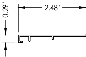
17 SIDELITE SPACER AFCO
