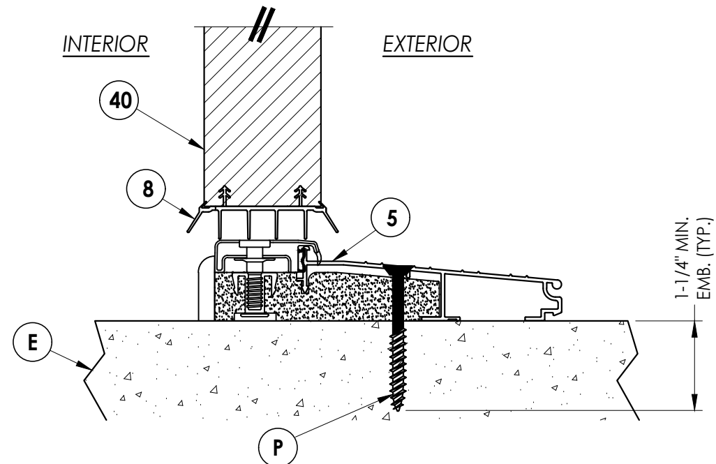
4 VERTICAL CROSS SECTION
