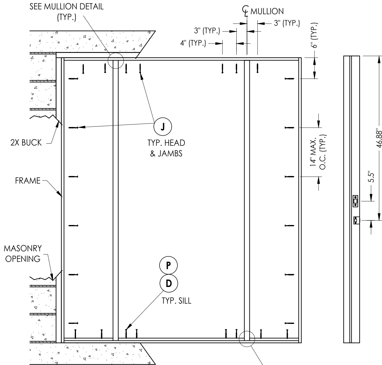
FRAME ANCHORING
