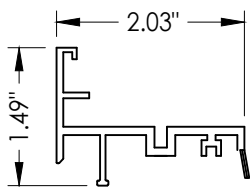
15 SIDELITE BASE AFCO
