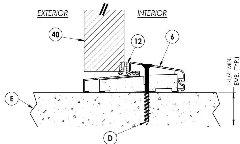
3 VERTICAL CROSS SECTION
