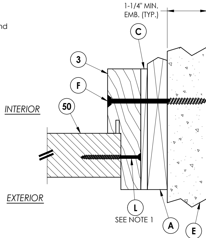
4 HORIZONTAL CROSS SECTION Shown w/ 1X sub-buck
