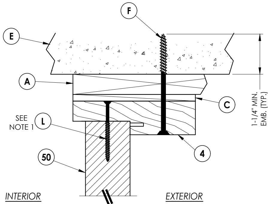
2 6 VERTICAL CROSS SECTION Shown w/1X sub-buck
