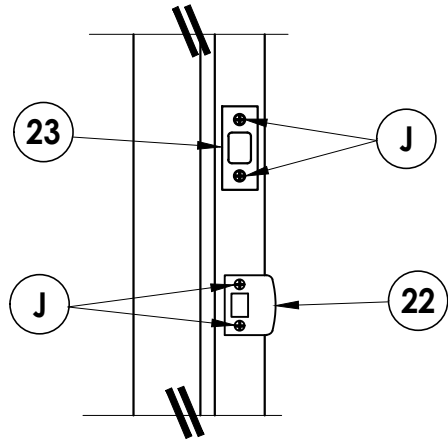
LATCH AND DEADBOLT DETAIL
