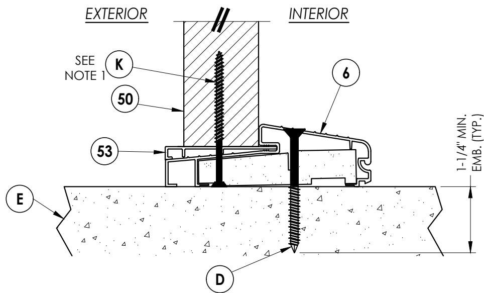
3 6 VERTICAL CROSS SECTION Outswing sill
