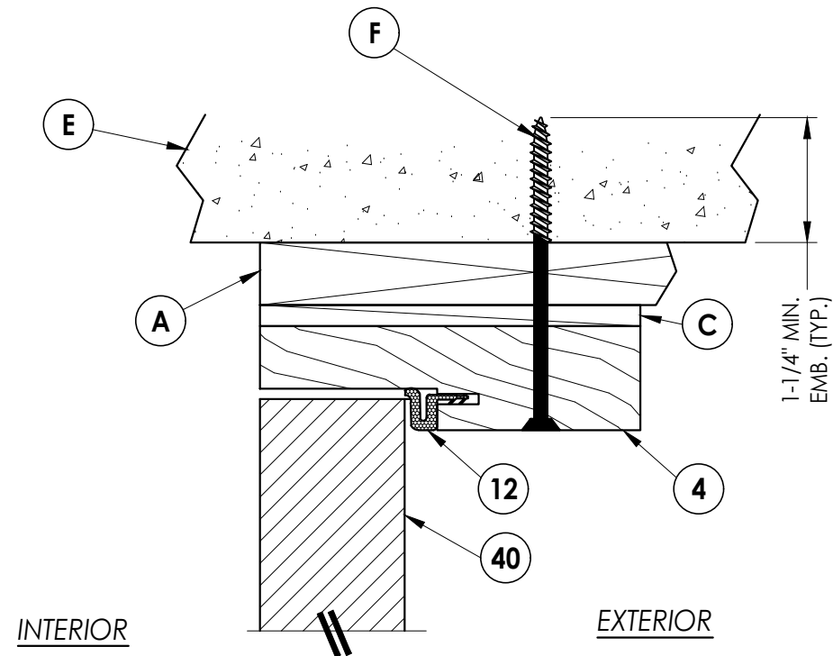
2 VERTICAL CROSS SECTION 5 Shown w/ 1X sub-buck
