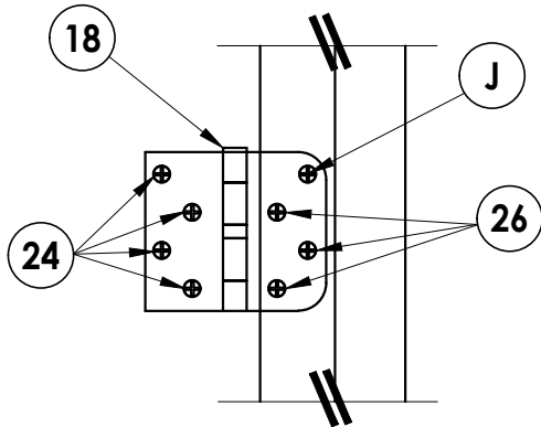
HINGE DETAIL
