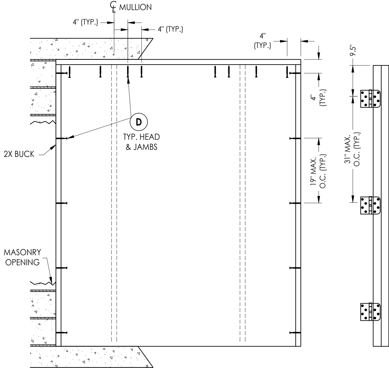
BUCK ANCHORING
