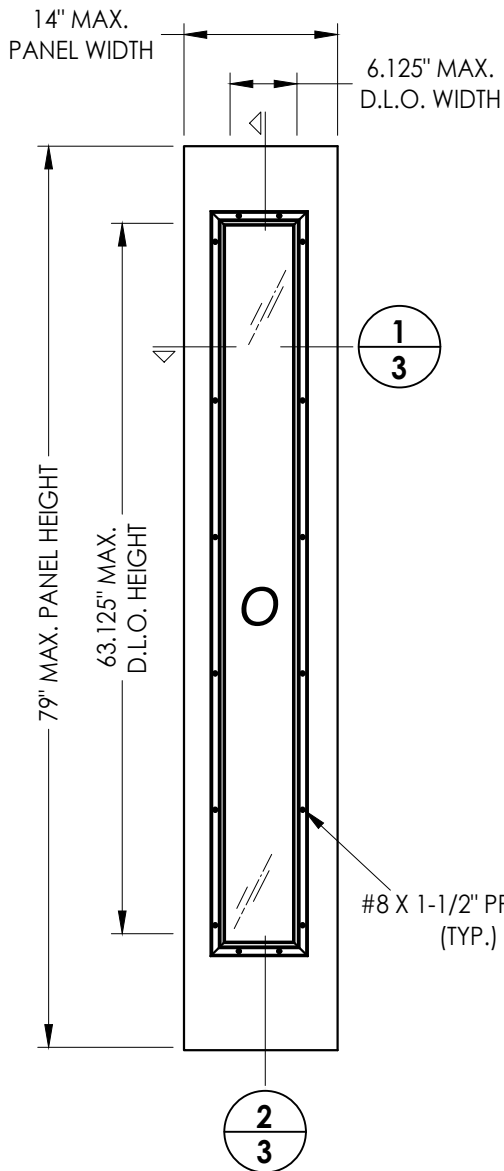
50 SIDELITE PANEL
