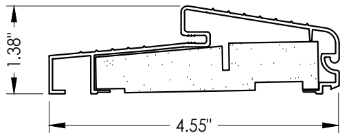
6 OUTSWING THRESHOLD AFCO
