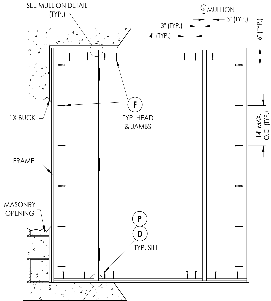
FRAME ANCHORING
