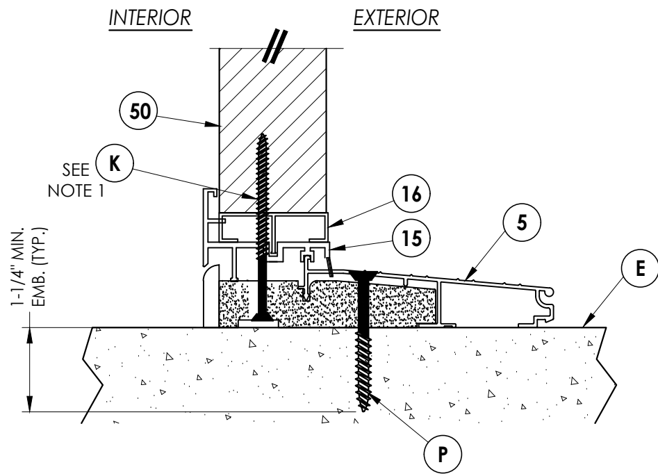
4 6 VERTICAL CROSS SECTION Inswing sill
