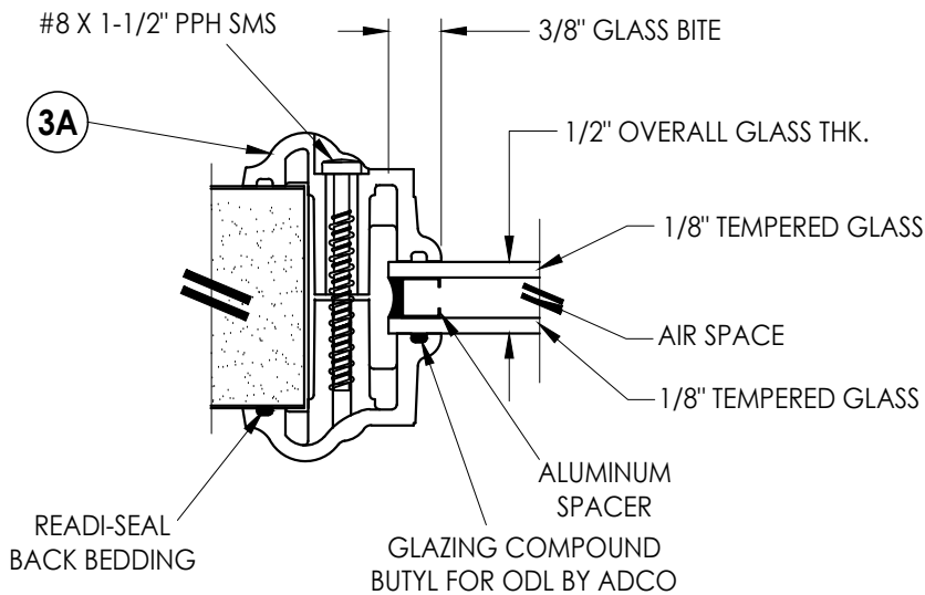
G1 GLAZING DETAIL ODL Lite Frame
